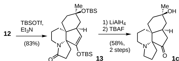
Scheme 6. Synthesis of 13-deoxyserratine ( 1c ).
