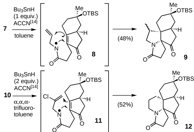
Scheme 5. Synthesis of pyrrolidine 9 and indolizidine 12 .
